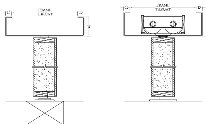
Typical head and floor section detail.
