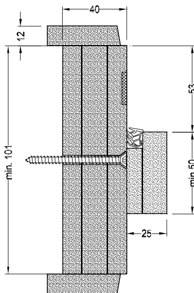
Euroseal frame profile - note hidden frame fixings
