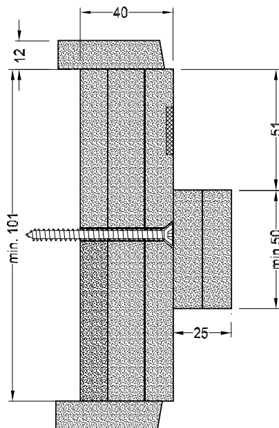
Typical frame profile - note hidden frame fixings
